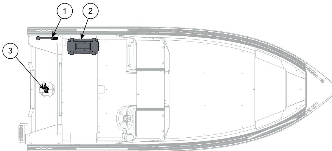
Figur 8.2 Buster S/S1/S2/Sc elektrisk utstyr
